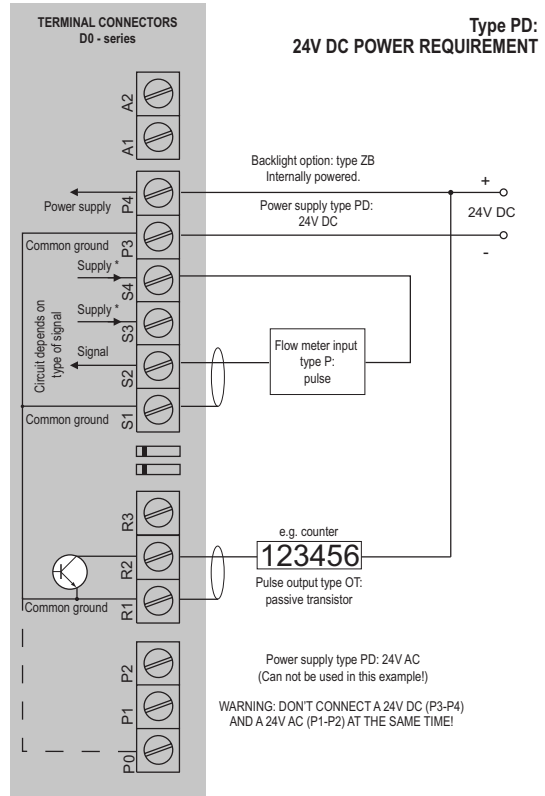
Configuration example D014-P-OT-PD-XX-ZB
