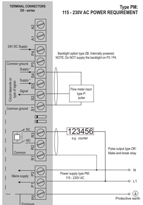
Configuration example D014-P-OR-PM-XX-ZB
