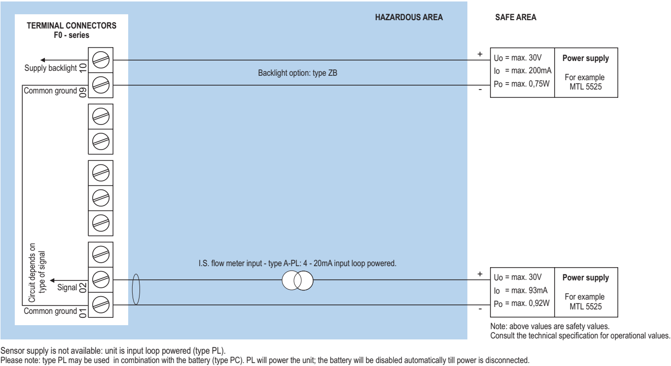
Configuration example IIA - IIB and IIC - F011-A-PX-XI-ZB - Basic power requirement 8 - 30V DC
