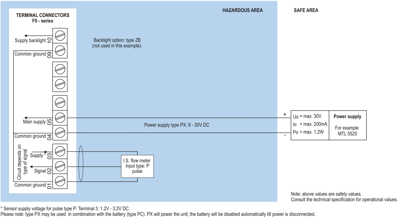
Configuration example IIA - IIB and IIC - F011-P-PX-XI-ZB - Basic power requirement 8 - 30V DC
