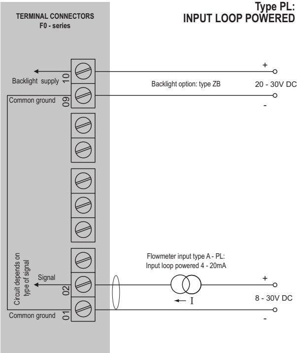
Configuration example F011-A-PL-XX-ZB
