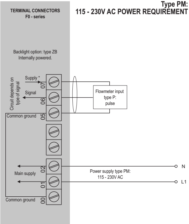
Configuration example F011-P-PM-XX-ZB
