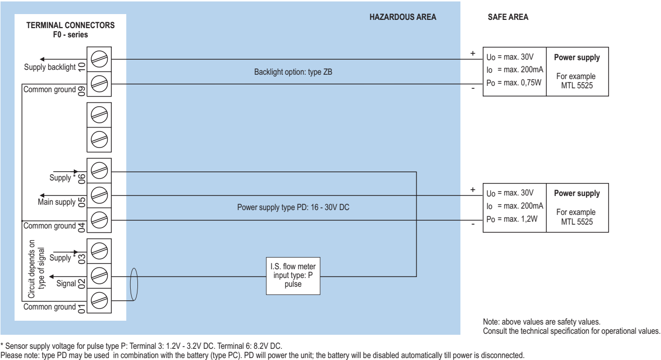
Configuration example IIA - IIB and IIC - F011-A-PD-XI-ZB - Power requirement 16 - 30V DC
